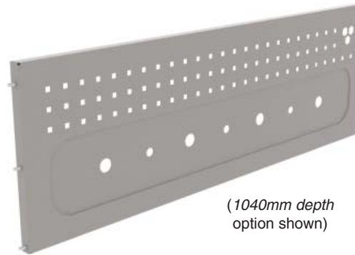
Tool Panels to be located inside end panels
